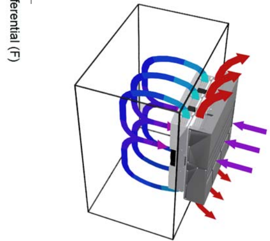
Air Flow Pattern
